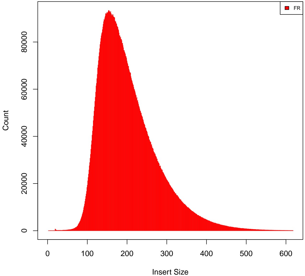
Insert Size Histogram for All_Reads in file alignment_sorted.bam
